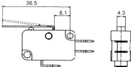
Standard lever
