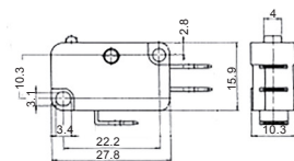
Standard lever
