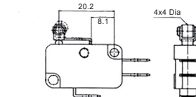
Standard roller
